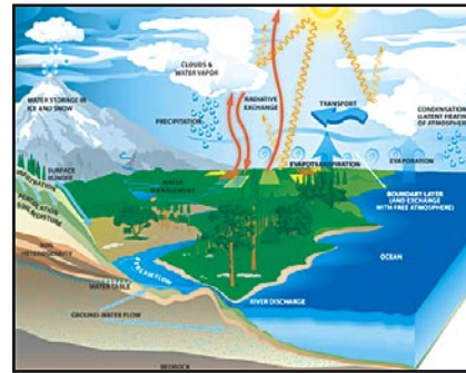
Figure 2.3. Hydrologic Cycle: Many impacts result from changes in land use and land cover in and beyond coastal watersheds.
