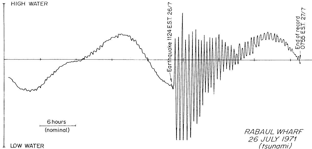
TSUNAMI EFFECT ON A TIDE GAUGE RECORD
